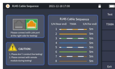
RJ45 Cable Sequence
